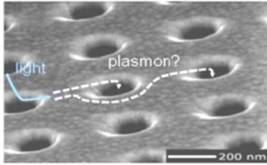
Figure 4 Initial surface-plasmon mechanism proposed to explain the EOT. The incident light first scatters into surface plasmons that subsequently propagate on the flat surface, couple to the hole and then tunnel the energy through the holes.
